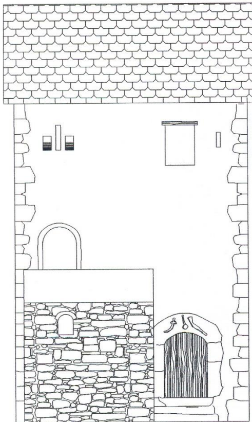
Drawing of Lalić Tower, M. Vrata, Ljubuški
